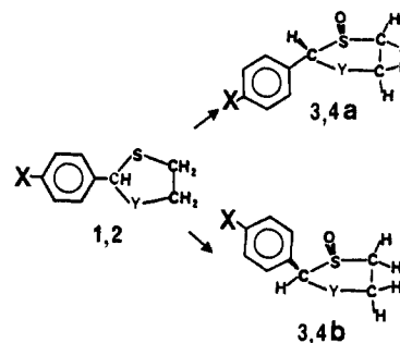
Scheme I. Oxidative (Bio)chemical Transformation of 2-( p -Methoxyphenyl)-1,3-dithiolane (1) and 2-( p -Cyanophenyl)-1,3-oxathiolane (2) to Their Corresponding Trans (a) and Cis (b) S -Oxides 3 and 4 a
